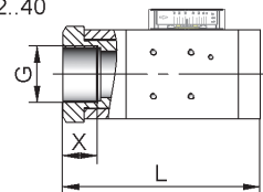
DN 32..40
